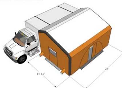
DOUBLE INFLATABLE AWNING SYSTEM
