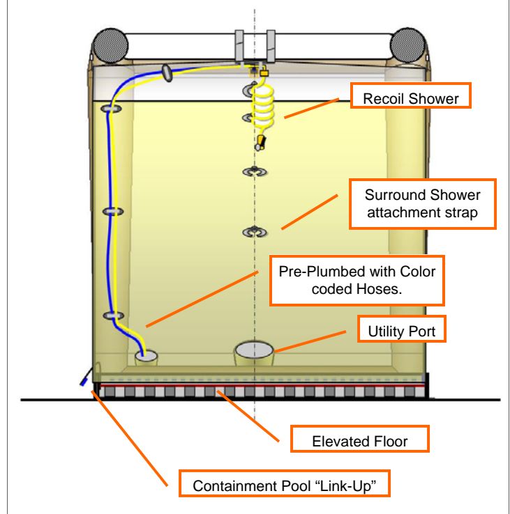
CROSS SECTION, INTERIOR VIEW
